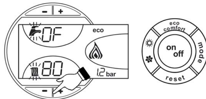
fig.24 - TEST mode
