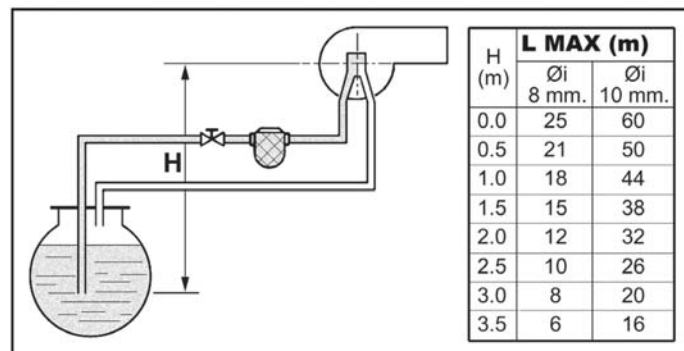
fig.20 – Suction feed
