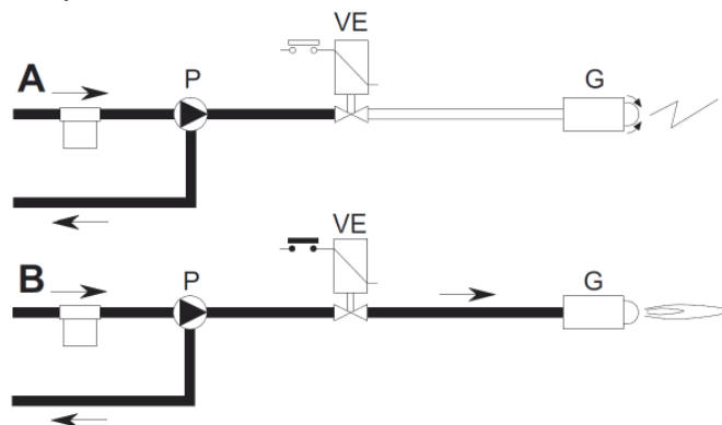
fig.30 - Starting
