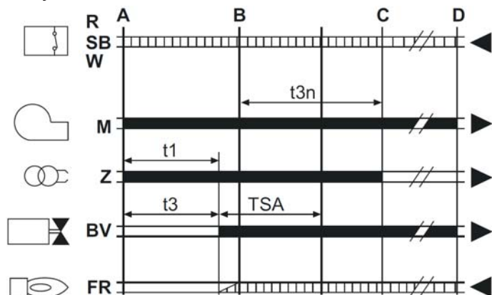
fig.31 - Unit cycle
