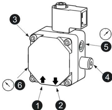
fig.26 - Bomba DANFOSS
