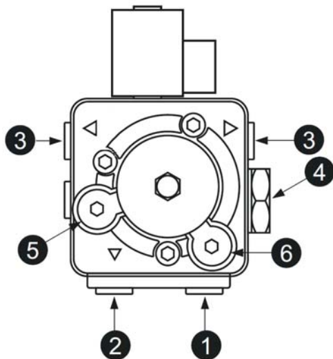
fig.25 - Pump ITALPUMP
