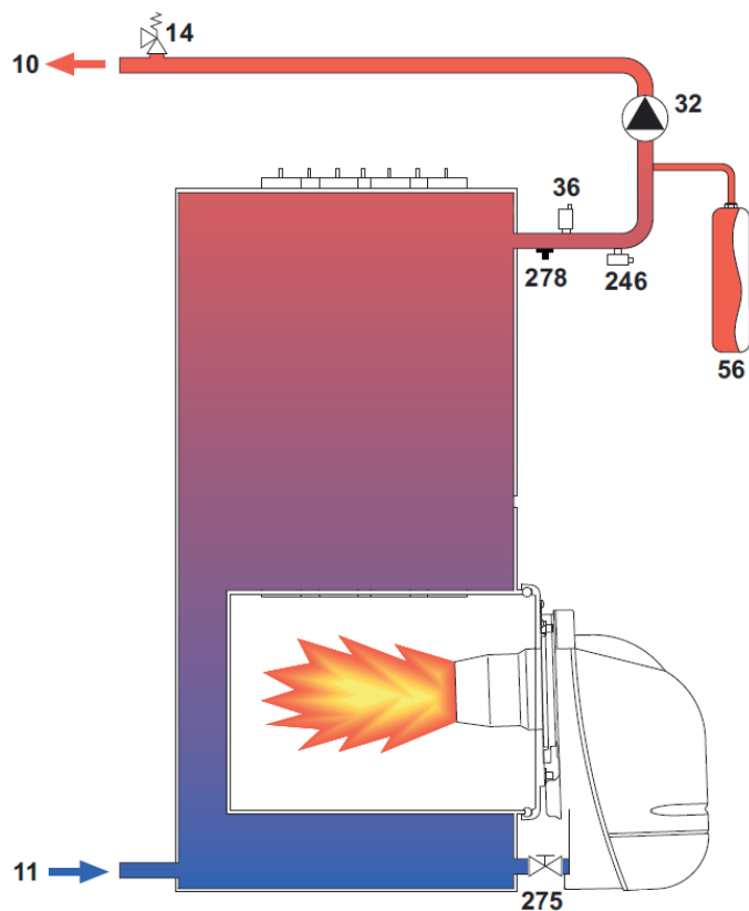
fig.38 - Water circuit
