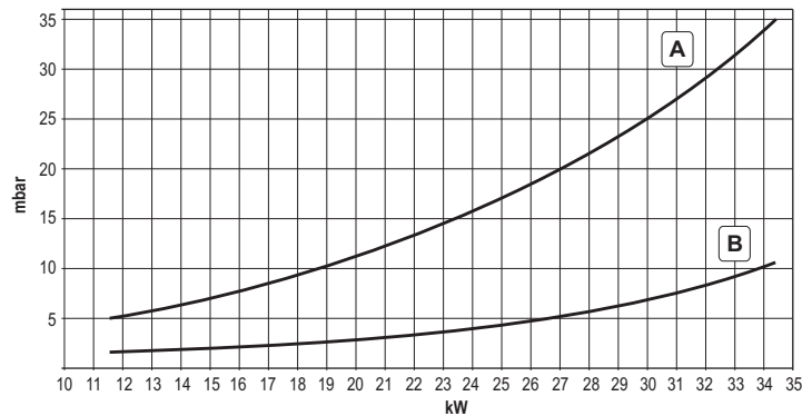
Pressure - power diagrams FL D C32
