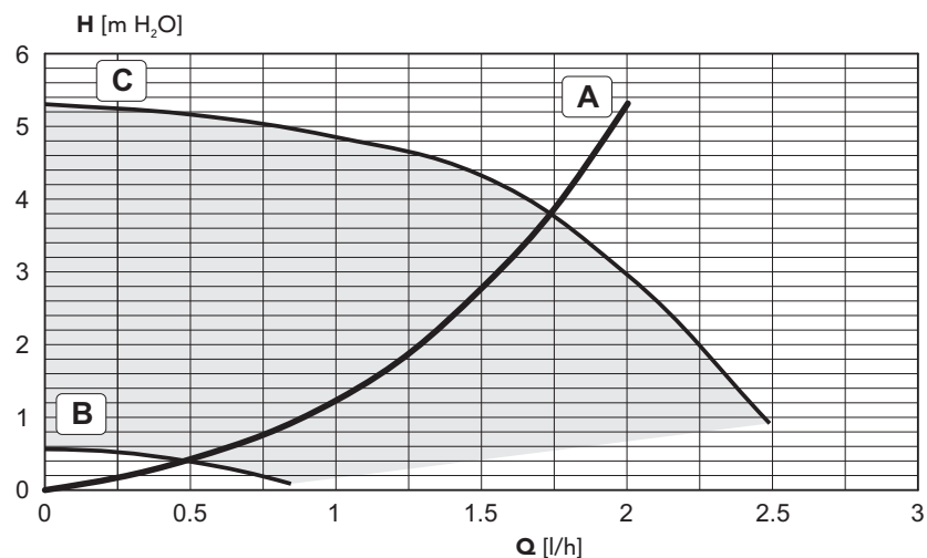
fig. 33 - Circulating pump head / pressure losses SILVER 34C
