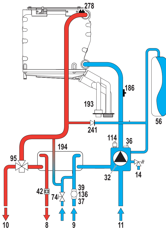
fig. 31 - Hydraulic circuit
