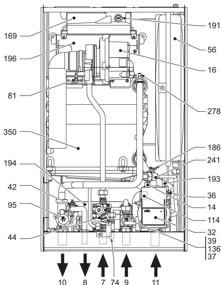
fig. 30 - General view
