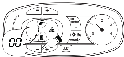
fig. 23 - TEST mode (heating power = 100%)
