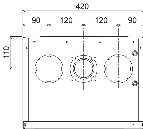
fig. 28 - Top view
