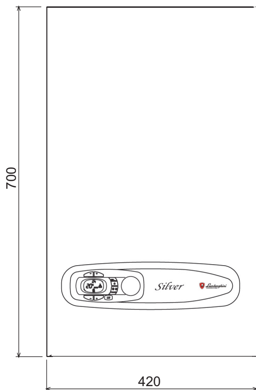
fig. 26 - Front view
