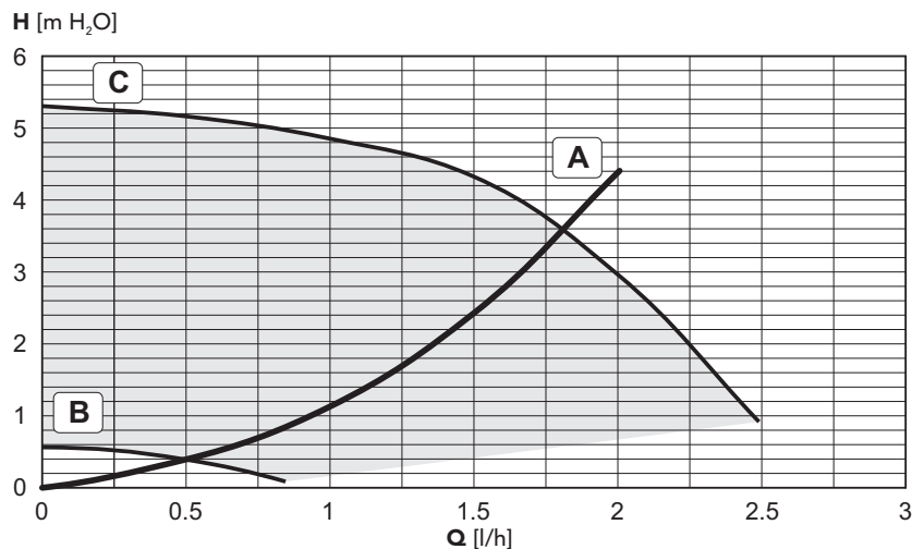
fig. 32 - Circulating pump head / pressure losses SILVER 24C
