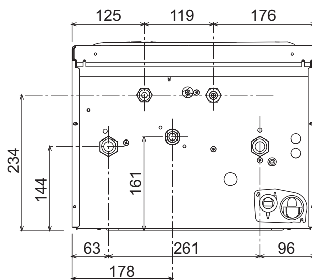
fig. 29 - Bottom view
