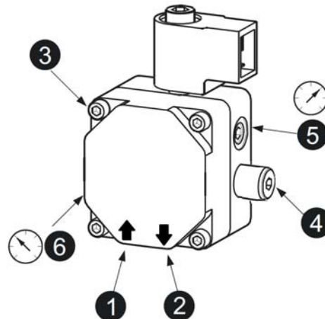
fig.27 - Pump DANFOSS
