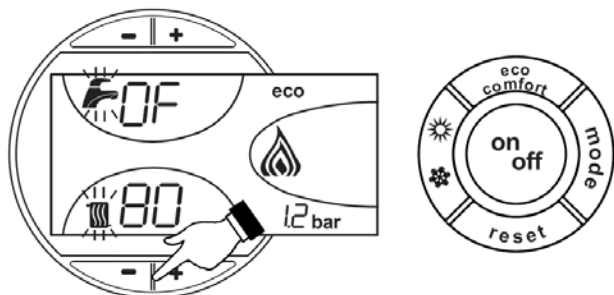
fig.25 - TEST mode
