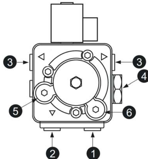
fig.26 - Pump ITALPUMP
