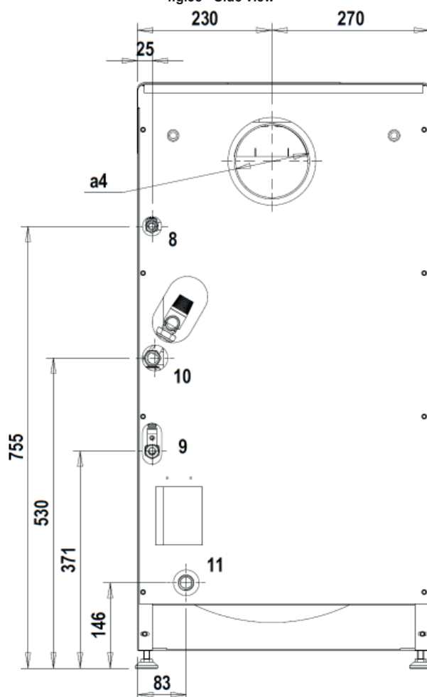
fig.39 - Rear view
