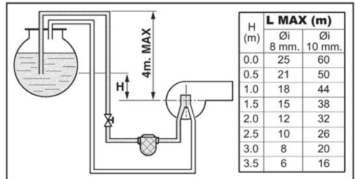
fig.22 - Siphon feed
