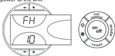
fig.6 - Boiler lighting
