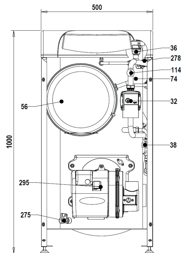
fig.37 - Front view
