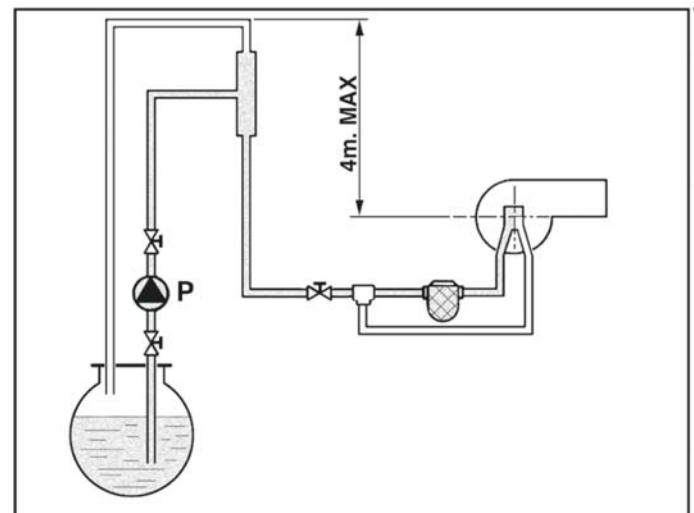
fig.23 - Ring feed
