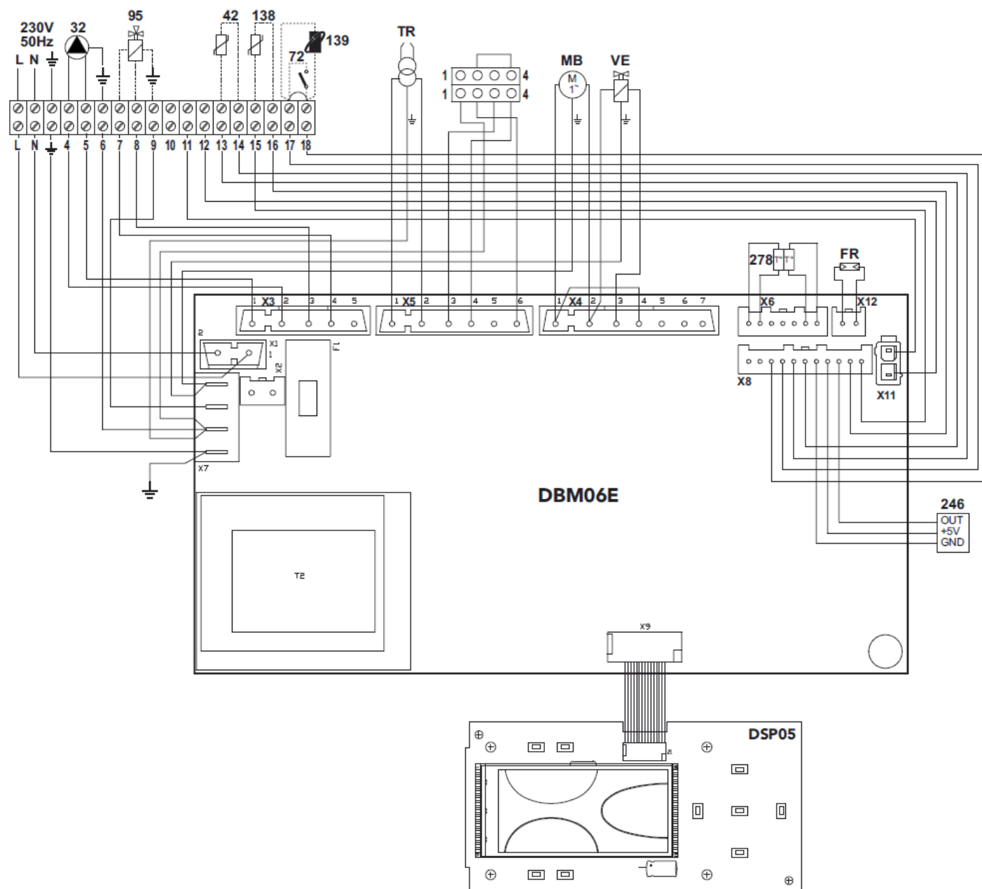
fig.43 - Wiring diagram
