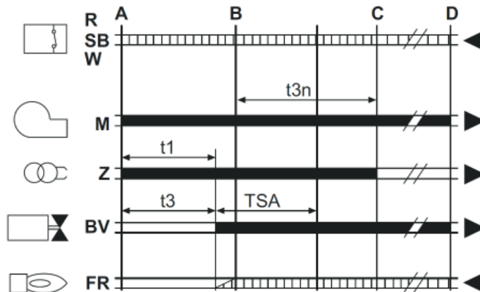
fig.32 - Unit cycle
