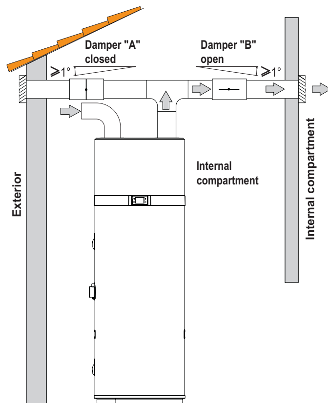
fig. 13 - Example of installation in the summer period
