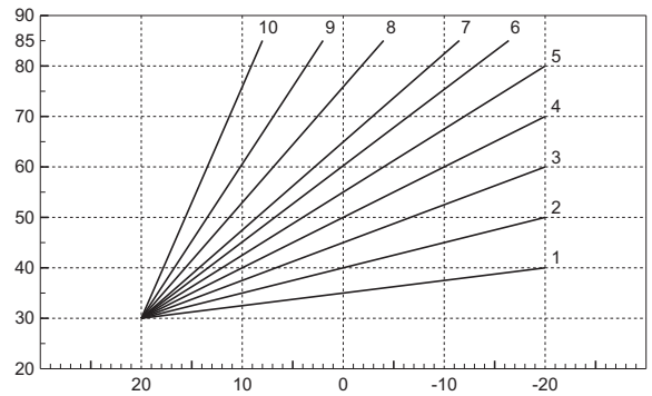
fig. 6 - Compensation curves
