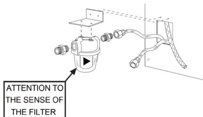
fig.19 – Fuel filter installation
