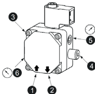
fig.27 - Bomba DANFOSS
