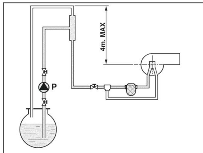
fig.22 – Ring feed
