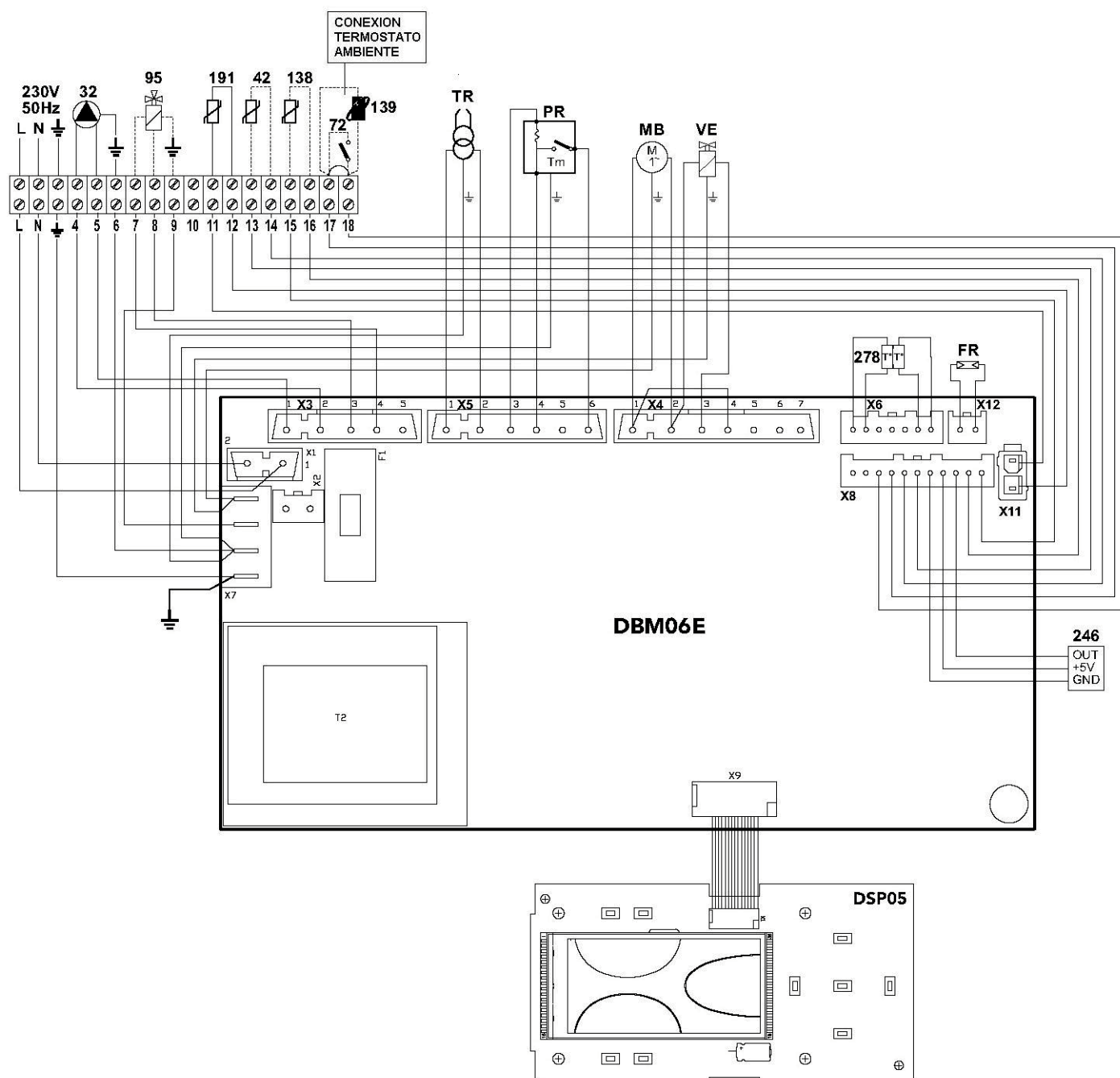
fig.43 – Wiring diagram
