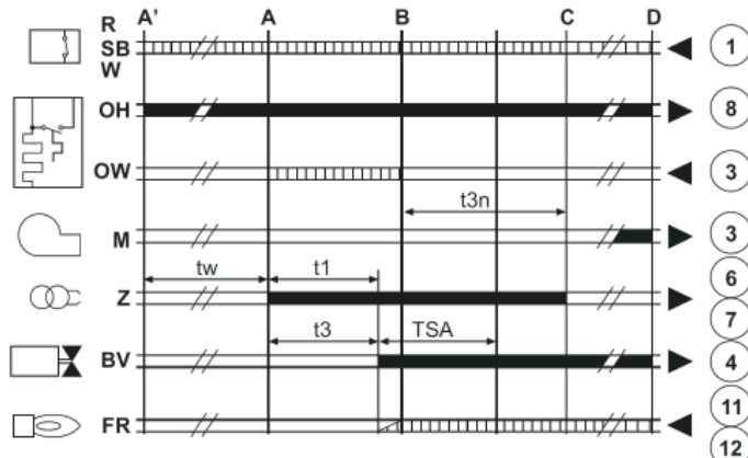
fig.32 - Unit cycle
