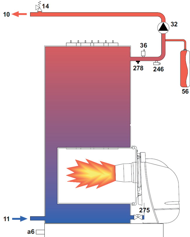
fig.40 – Water circuit
