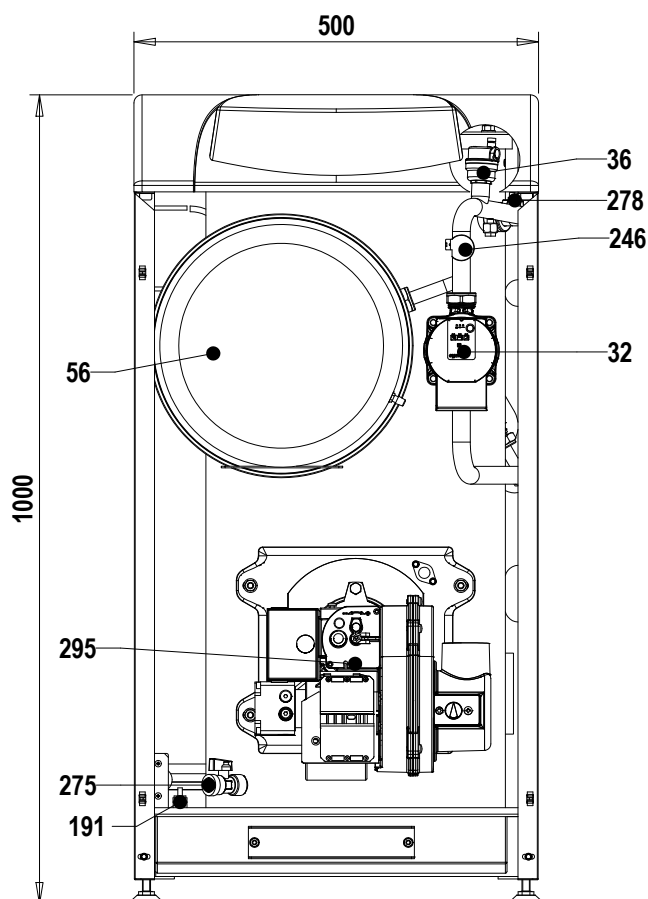
fig.38 – Front view
