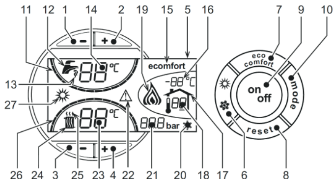
fig.1 – Control panel
