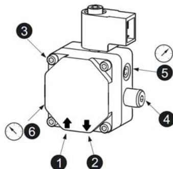
fig.27 - Pump DANFOSS
