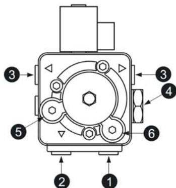
fig.26 - Pump ITALPUMP
