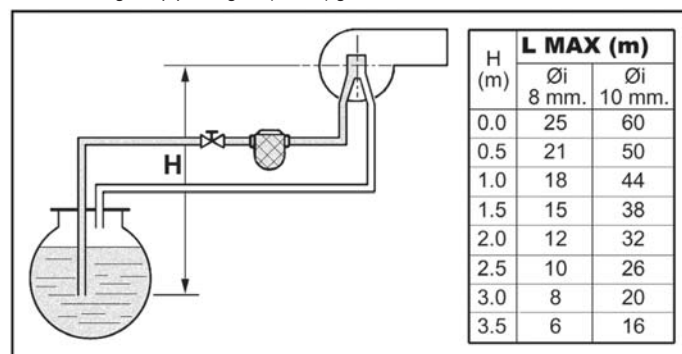
fig.20 – Suction feed
