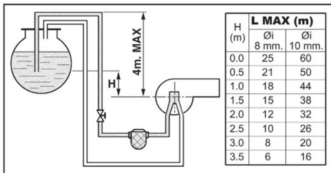
fig.21 – Siphon feed
