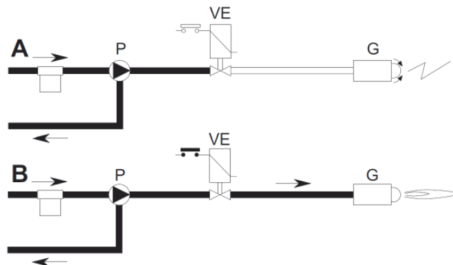
fig.31 - Starting
