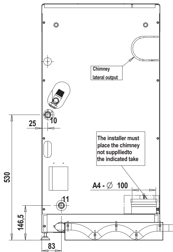
fig.39 – Rear view
