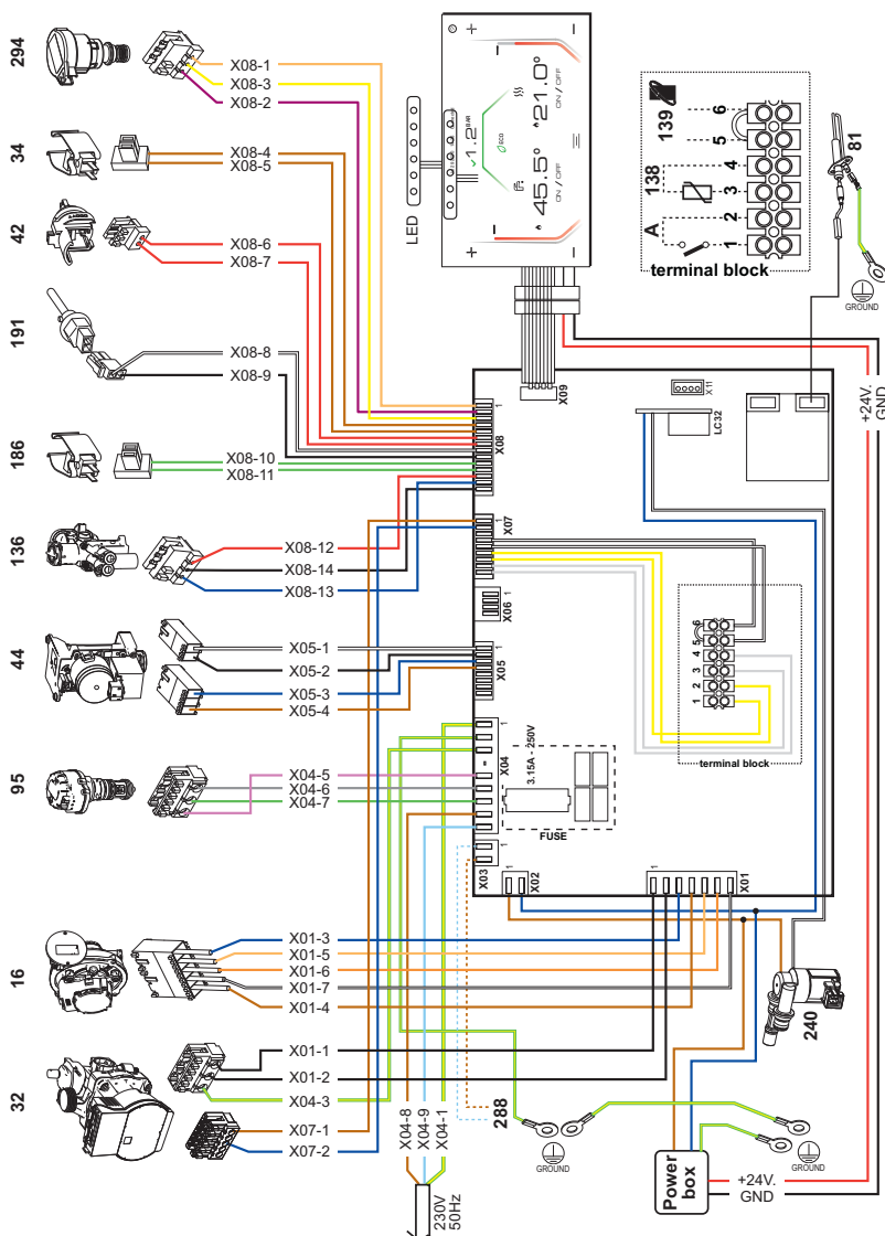
fig. 58- Wiring diagram
