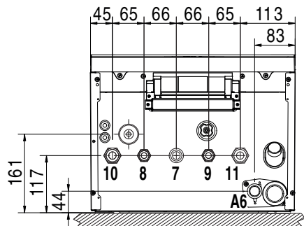
fig. 50- Bottom view
