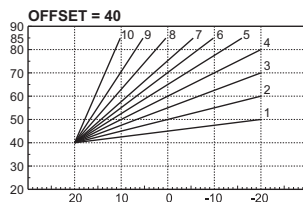
fig. 38- Example of compensation parallel curve offset
