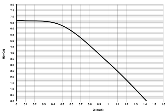
fig. 56- Residual head available for system
