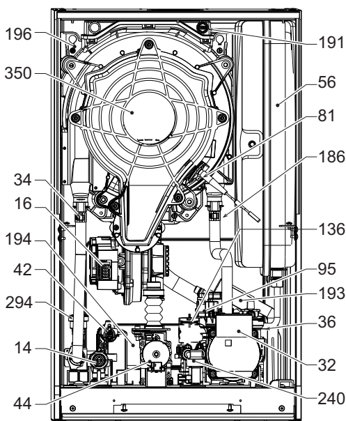
fig. 54- General view
