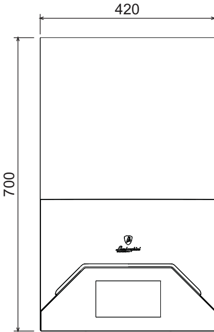
fig. 47- Front view
