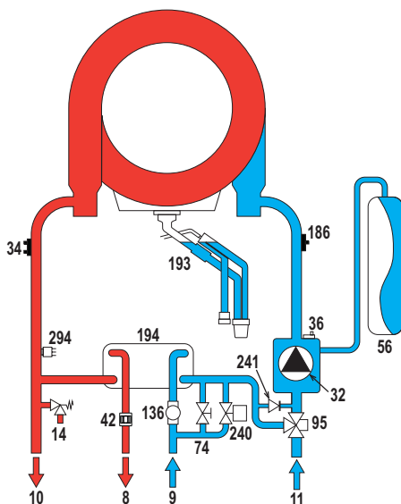
fig. 55- Hydraulic circuit
