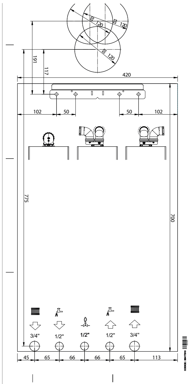
fig. 53- Paper template
