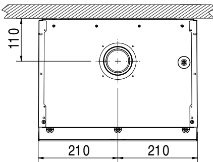
fig. 49- Top view
