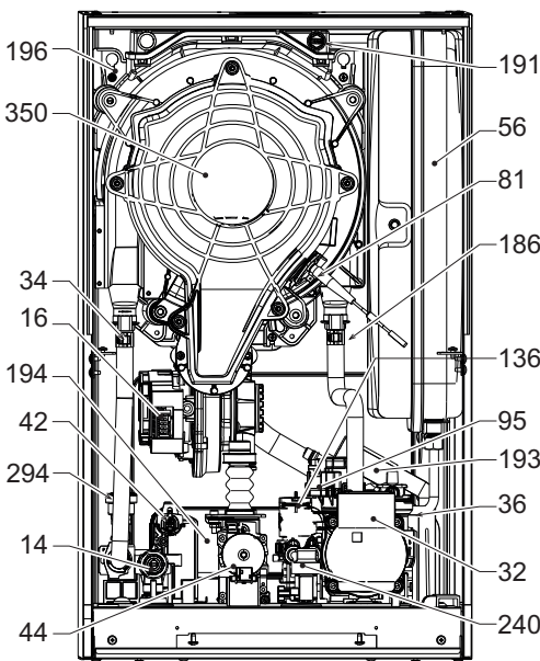
fig. 54- Vista general
