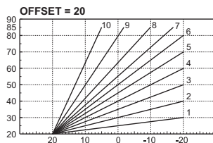
fig. 37- Compensation curves
