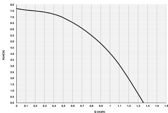
fig. 57- Residual head available for system
