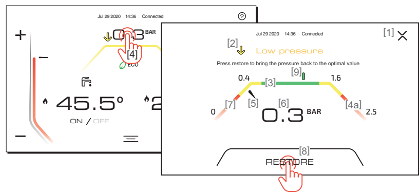
fig. 8- Pressure control
