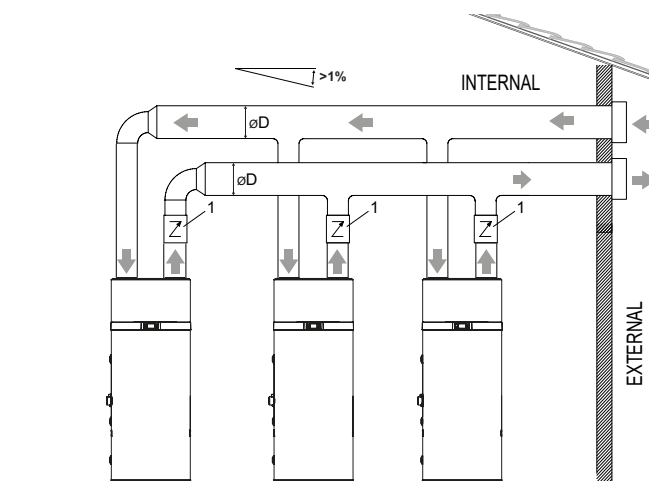
fig. 55- Example of air outlet connection
