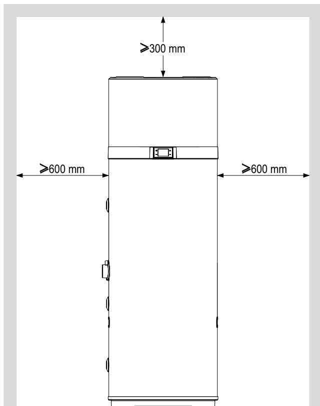
fig. 48 - Minimum spaces
