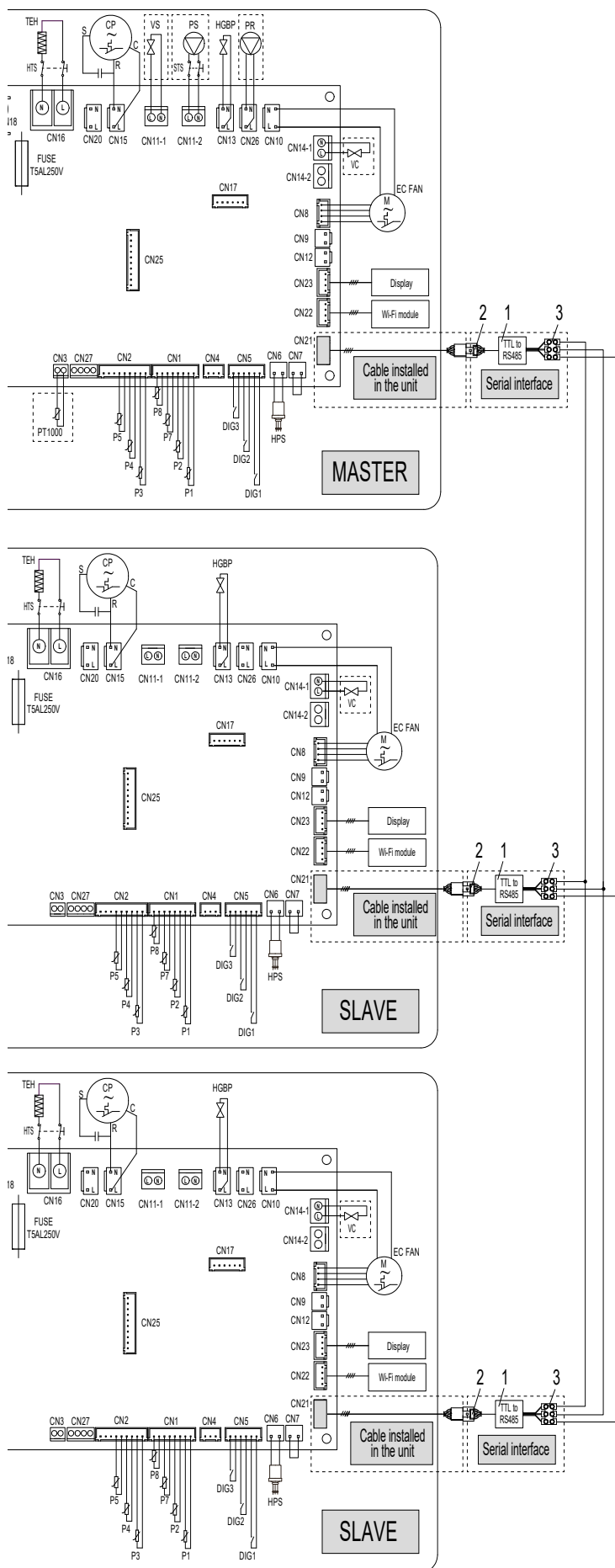
fig. 74 - Cascade wiring diagram
